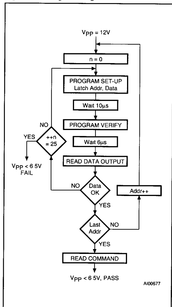
Figure 13. Programming Flowchart
