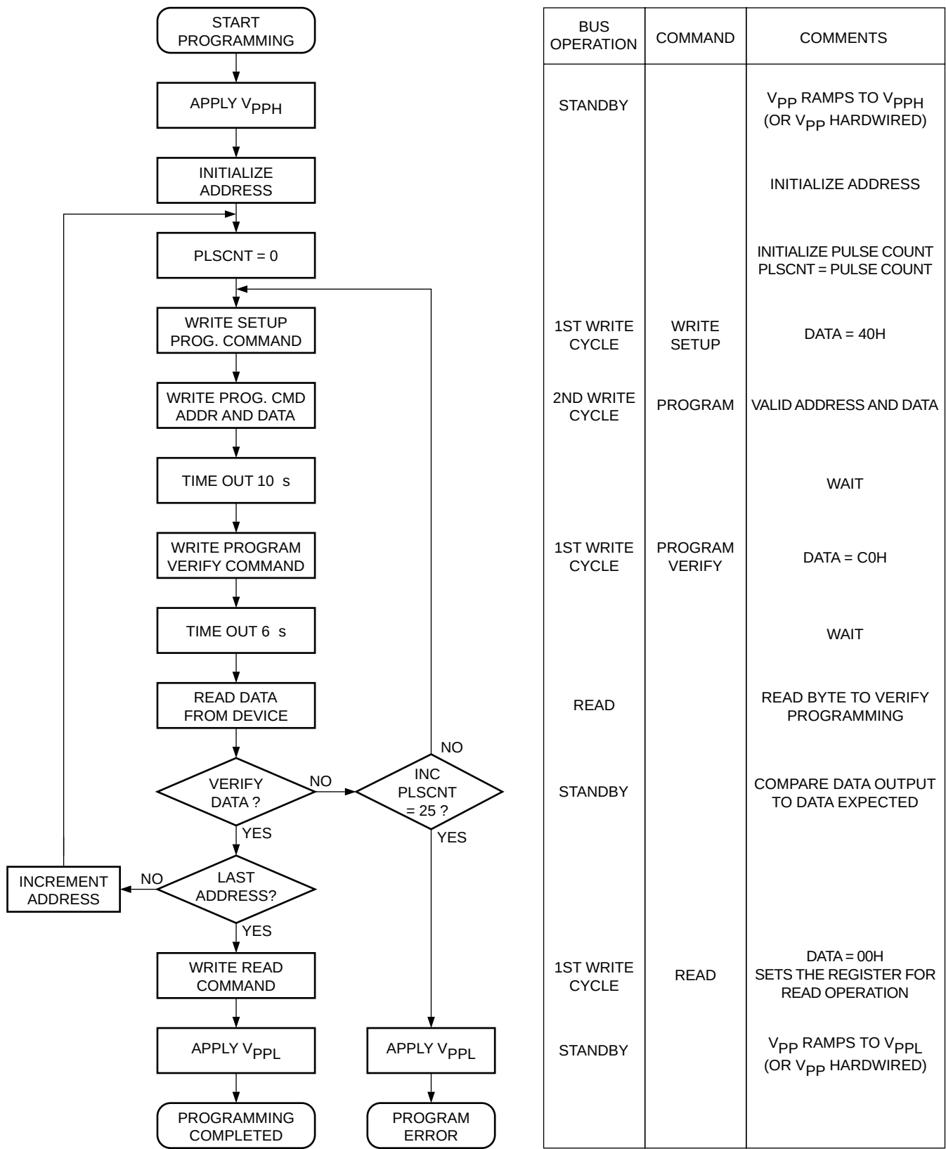
Figure 7. Programming Algorithm(1)
