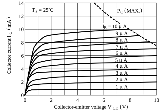
Fig.5-b Collector Current vs. Collector-emitter Voltage (PT510)
