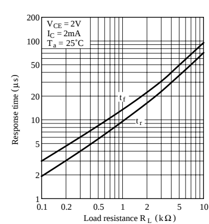
Fig. 7 Response Time vs. Load Resistance
