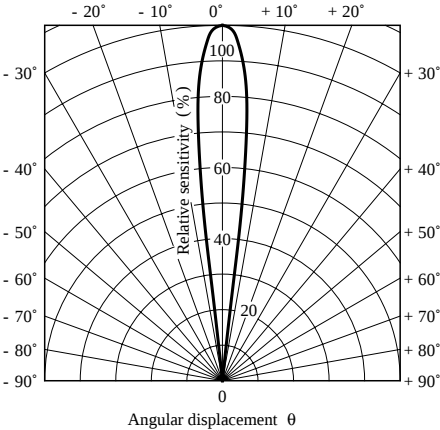
Fig. 9 Sensitivity Diagram ( T_a = 25^{\circ}\text{C} )
