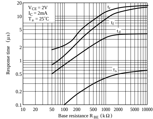
Fig. 8 Response Time vs. Base Resistance (PT510)
