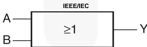
Figure 2. Logic Symbol
