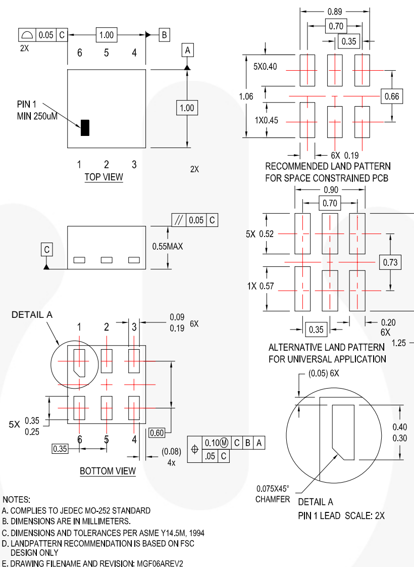
Figure 9. 6-Lead, MicroPak2, 1x1mm Body, .35mm Pitch
