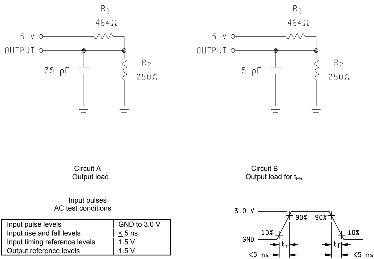
FIGURE 4. Output load circuit and test conditions.
