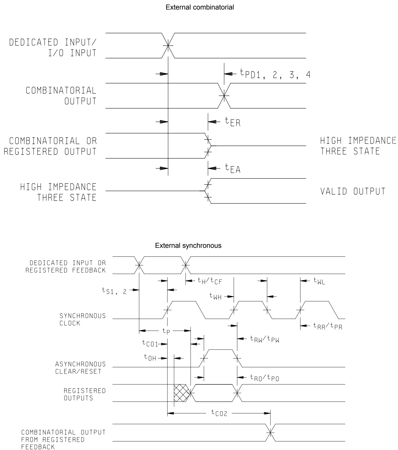
FIGURE 5. Switching waveforms.
