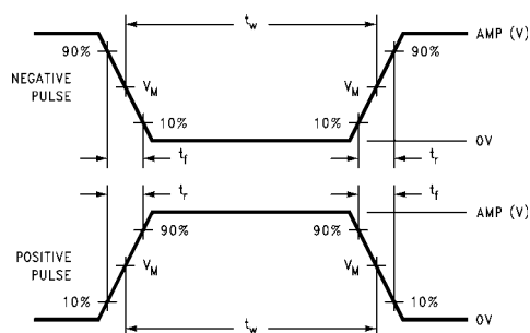
FIGURE 2. V_M = 1.5V
