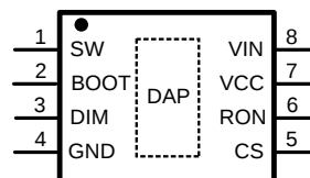
Figure 2. 8-Lead Plastic So PowerPAD-8 Package
