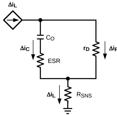
Figure 22. LED and C O Ripple Current
