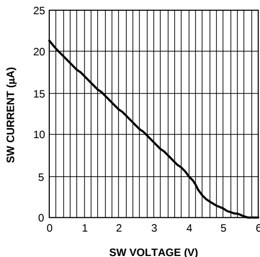
Figure 23. LED Current From SW Pin
