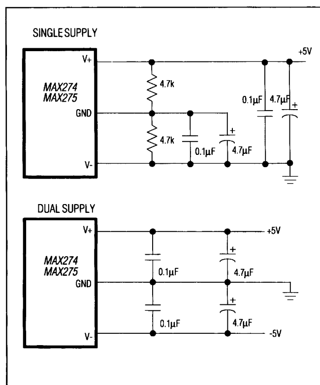
Figure 9. Power-Supply Configurations
