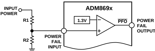
Figure 7. Power Fail Comparator
