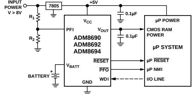
Figure 22b. ADM8690/ADM8692/ADM8694 Typical Application Circuit B
