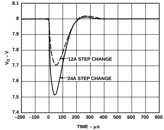
Figure 19. Predicted Response to 12\text{ A} and 24\text{ A} Step Change in Load Current, di/dt = 12\text{ A}/\mu\text{s} , for C_{LOAD} = 1000\text{ }\mu\text{F} and R_{ESR} = 10\text{ m}\Omega
