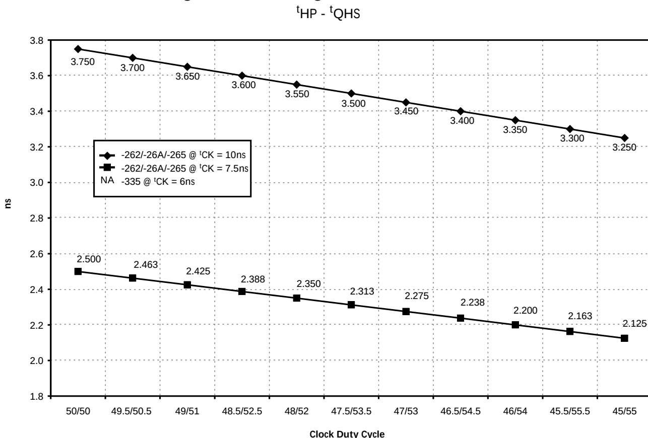
Figure 8: Derating Data Valid Window
