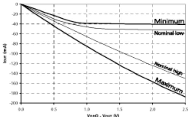
Figure 10: Pull-Up Characteristics
