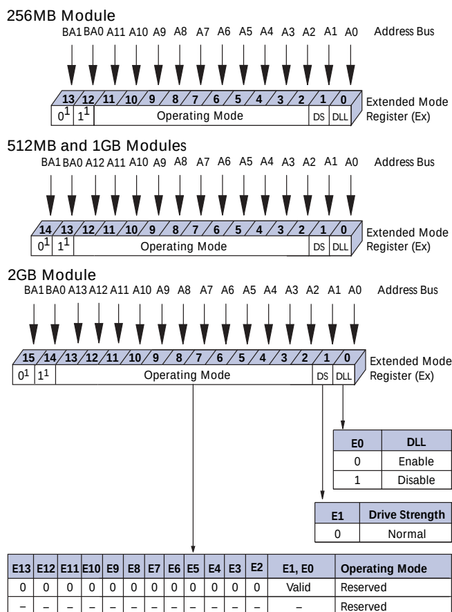
Figure 7: Extended Mode Register Definition Diagram
