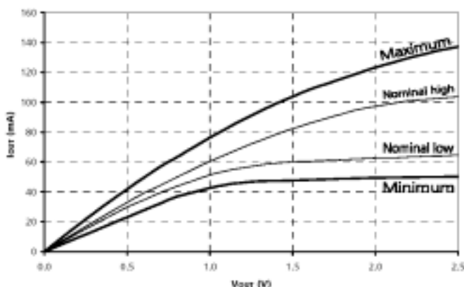
Figure 9: Pull-Down Characteristics
