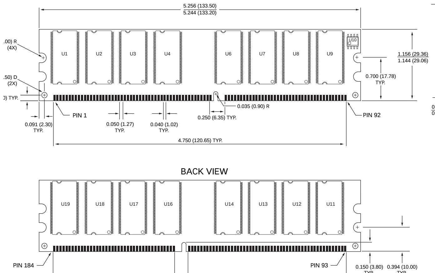
Figure 18: 184-PIN DDR DIMM Dimensions – Low-Profile PCB
