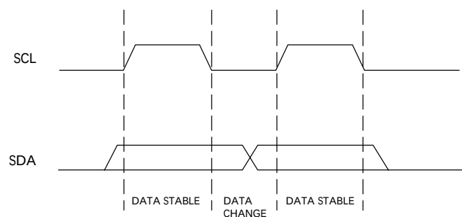
Figure 13: Data Validity
