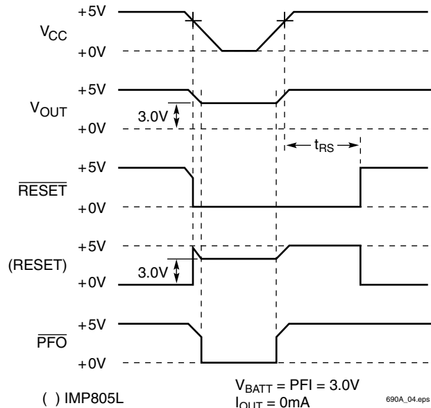
Figure 2. Timing Diagram
