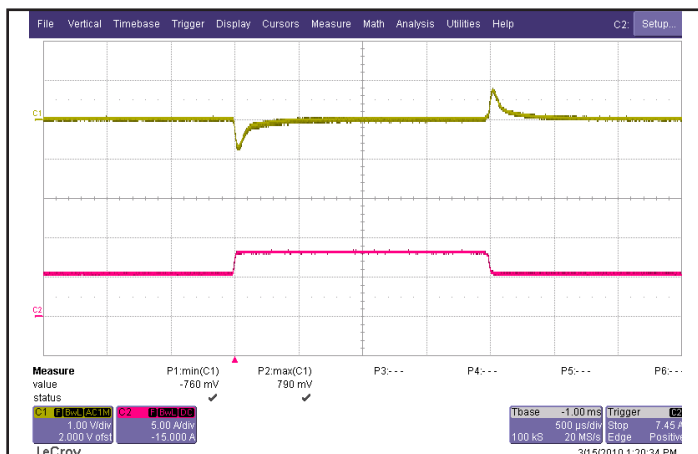
Figure 5: Output voltage response to step-change in load current (50%-75%-50% of I out (max); dI/dt = 0.1A/μs). Load cap: 15μF tantalum cap and 1μF ceramic cap. Ch 1: V out (1V/div), Ch 2: I out (5/div).
