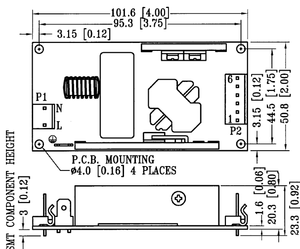
SINGLE OUTPUT
