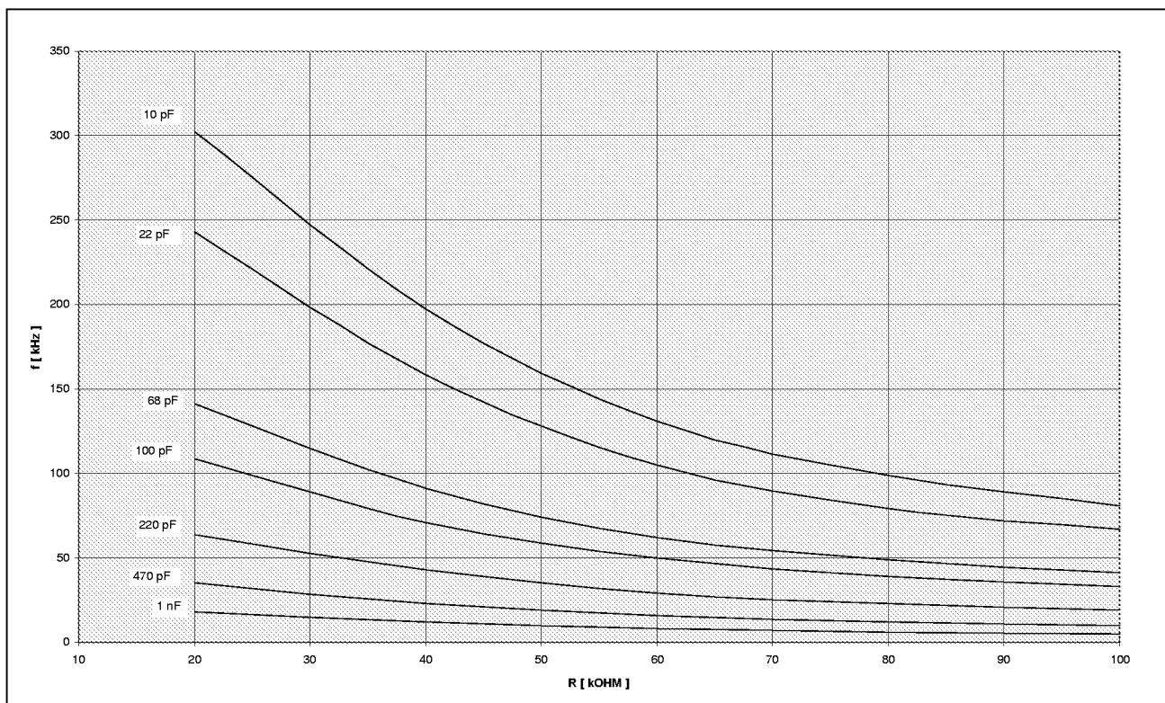
Figure 8 Switching Frequency
