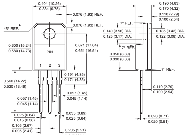
TO-220AB
