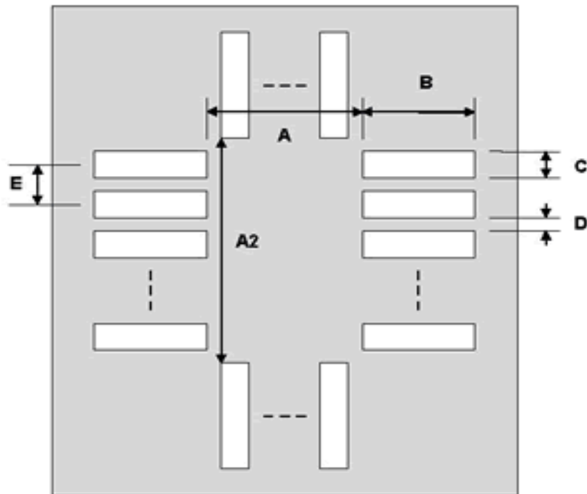
Top View (SMT Footprint)
