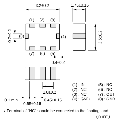
LFL32 Series
