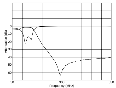
Frequency Characteristics
