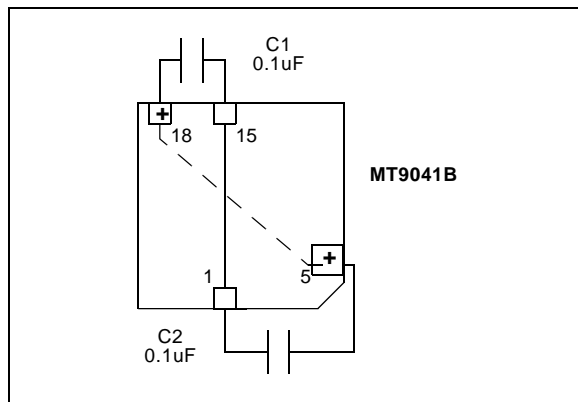
Figure 8 - Power Supply Decoupling
