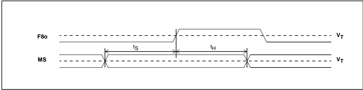
Figure 13 - Input Controls Setup and Hold Timing
