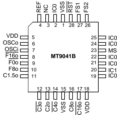
Figure 2 - Pin Connections
