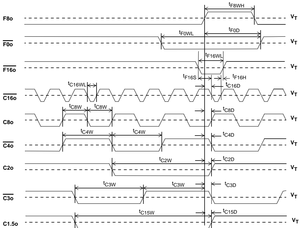
Figure 12 - Output Timing 1
