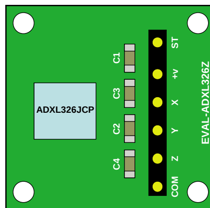
Figure 2. Layout
