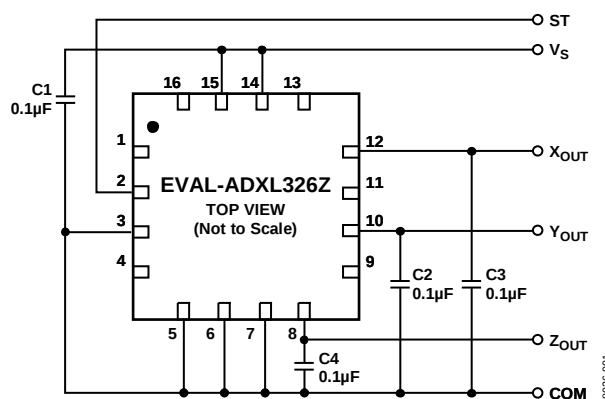
Figure 1. Schematic
