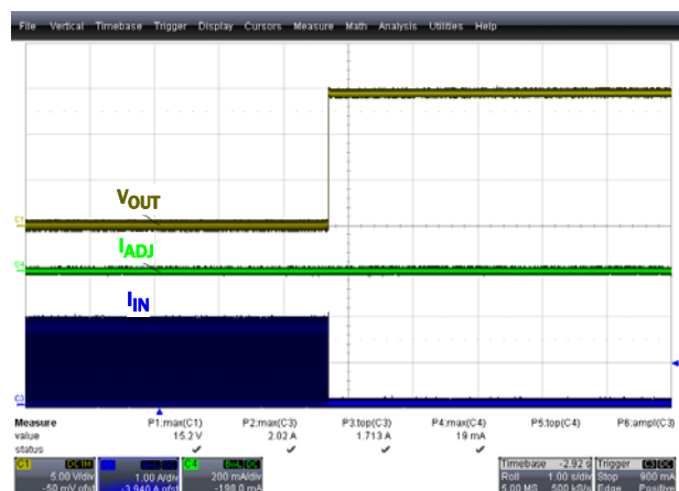
FIGURE 20. SHORT-CIRCUIT RECOVERY
