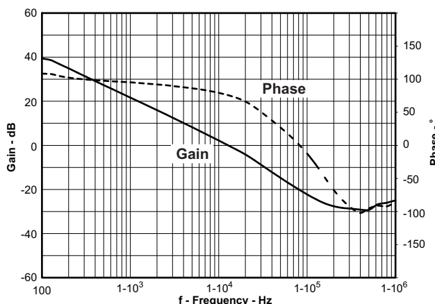
Figure 6. TPS54060EVM-457 Loop Response
