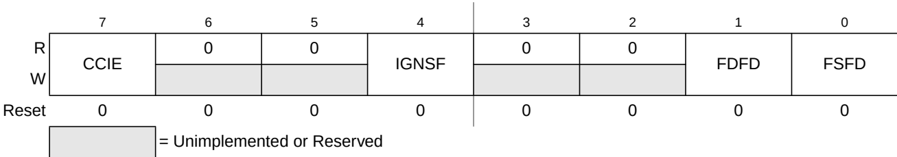
Figure 15-9. Flash Configuration Register (FCNFG)
