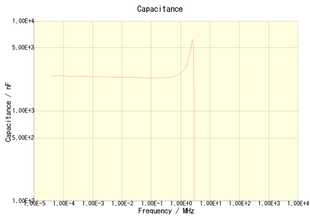
C3216X7R1E225K160AA
