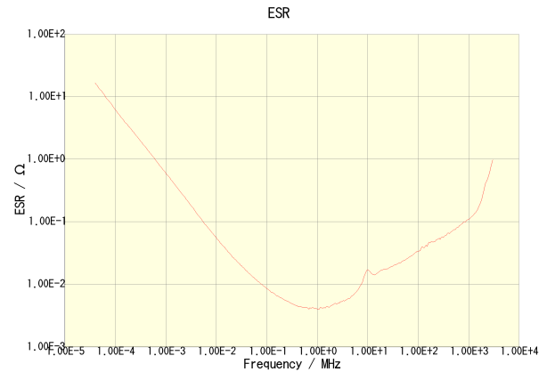
C3216X7R1E225K160AA
