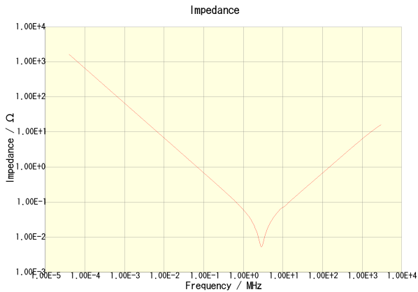
C3216X7R1E225K160AA
