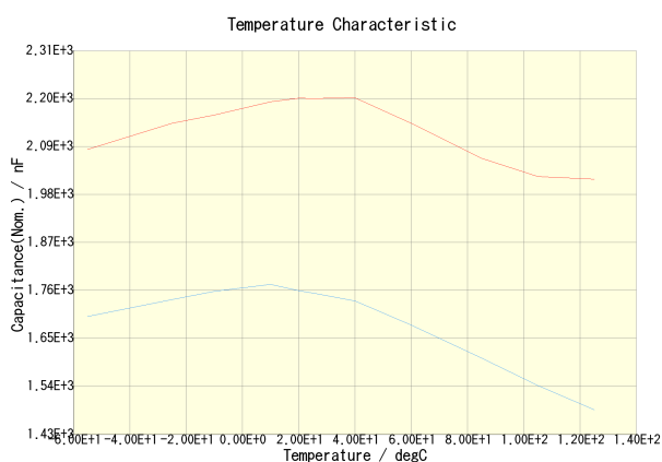
C3216X7R1E225K160AA(DC Bias = 0V) C3216X7R1E225K160AA(DC Bias = 12.5V)
