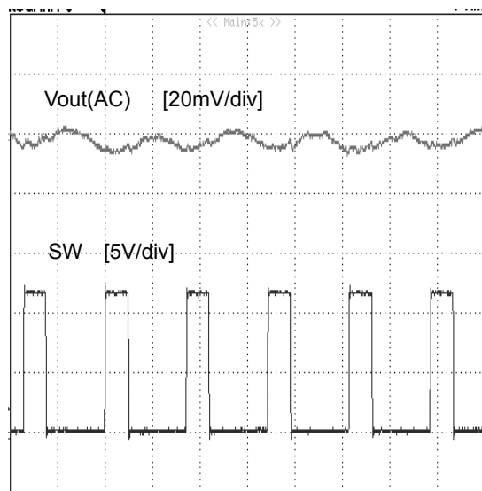
Figure 6. V_{out} Ripple ( V_{IN}=12V , V_{out}=3.3V , L=4.7\mu H , C_{out}=44\mu F , I_{out}=0A )
