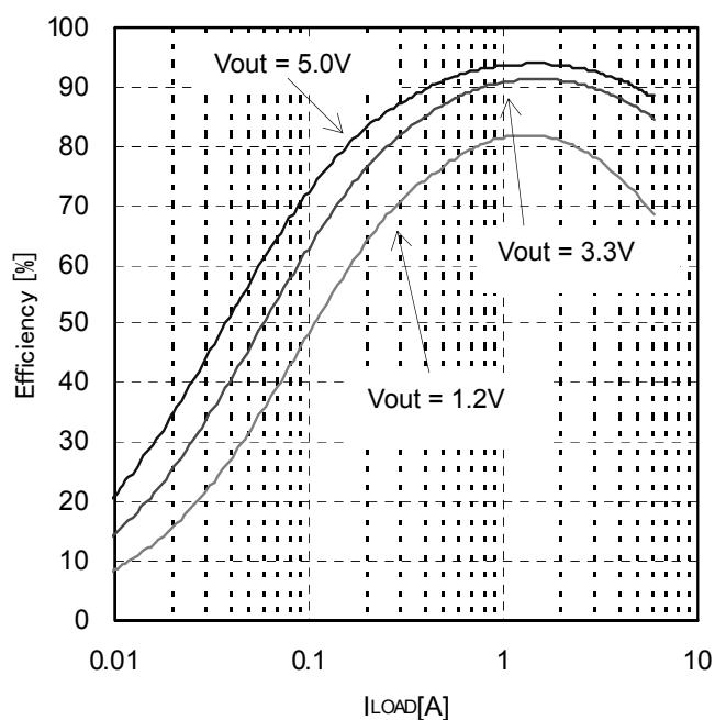
Figure 4. Efficiency ( V_{IN}=12V , L=3.3/4.7/4.7\mu H ( V_{out}=1.2/3.3/5.0V ), C_{out}=44\mu F )
