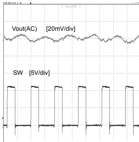
Figure 7. V_{out} Ripple ( V_{IN}=12V , V_{out}=3.3V , L=4.7\mu H , C_{out}=44\mu F , I_{out}=5A )
