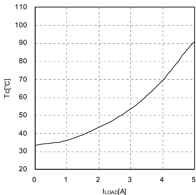
Figure 5. T_c - I_{LOAD} ( V_{IN}=12V , V_{out}=3.3V , L=4.7\mu H , C_{out}=44\mu F )
