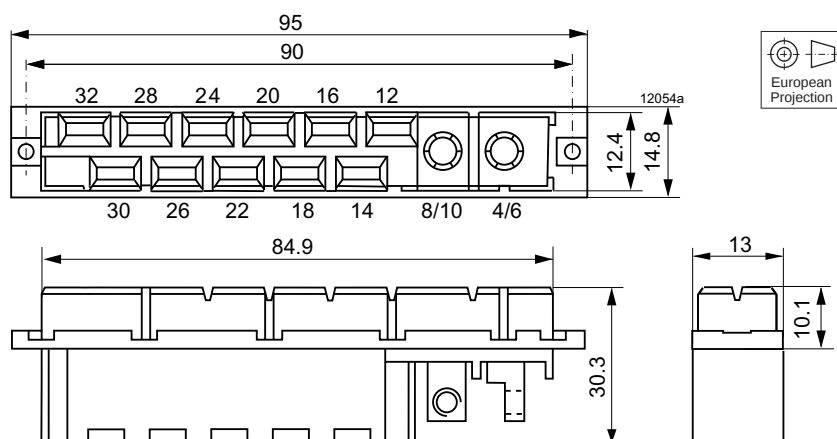
Fig. 12 STV-H15 S2-FSF/CO 11 faston terminals and two screw jacks.
