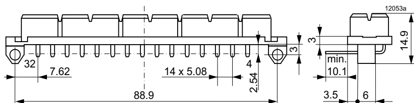
STV-H15-FWS/CO, solder pins for PCB mounting
