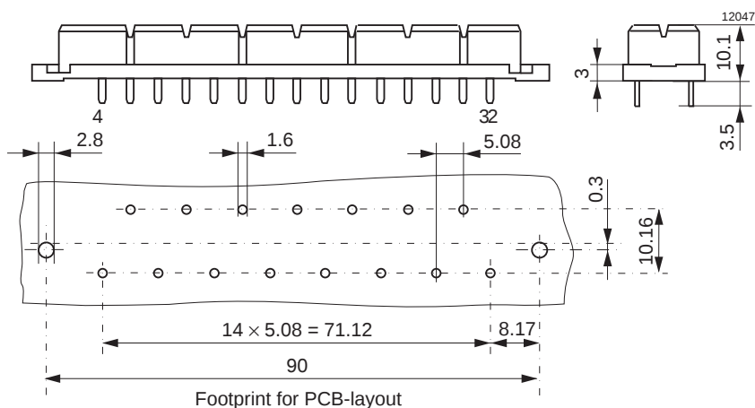
STV-H15-FB/CO, solder pins
