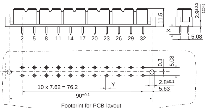
Fig. 5 STV-H11-FB/CO-G, solder pins X = 5.2 Y = \varnothing 1.6 STV-H11-FBG/CO, solder pins X = 5.2 Y = \varnothing 1.6 STV-H11-FBER/CO, solder pins X = 4.3 Y = \varnothing 1.0 STV-H11-FP/CO, press insert pins X = 6.5 Y = \varnothing 1.0
