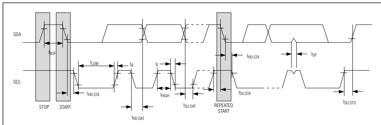
Figure 6. Timing Diagram
