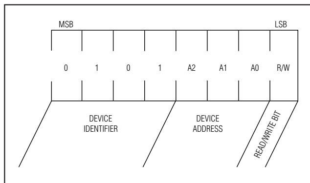
Figure 3. Control Byte
