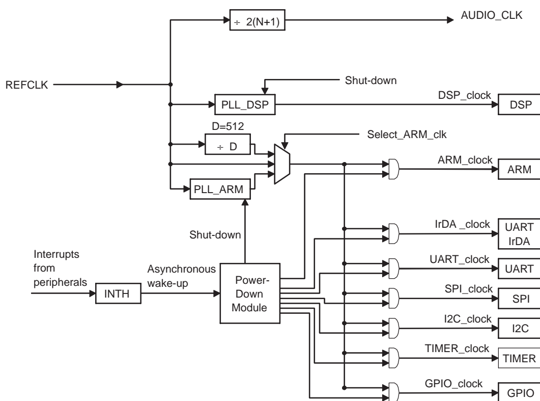
Figure 4–2. Clock Management Module
