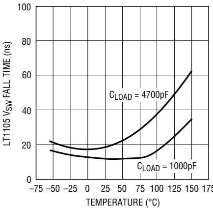
LT1105 V_{SW} Fall Time vs Temperature
