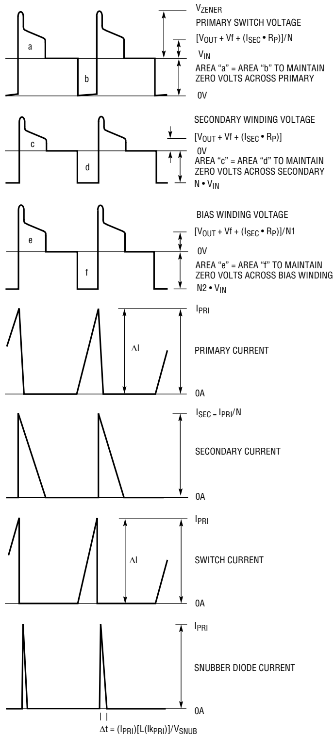
Flyback Waveform for Discontinuous Mode Operation
