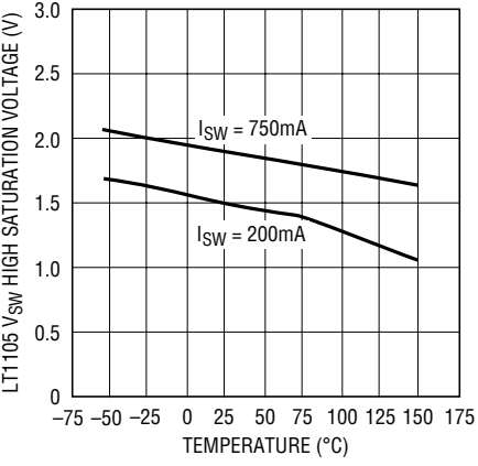
LT1105 V_{SW} High Saturation Voltage vs Temperature
