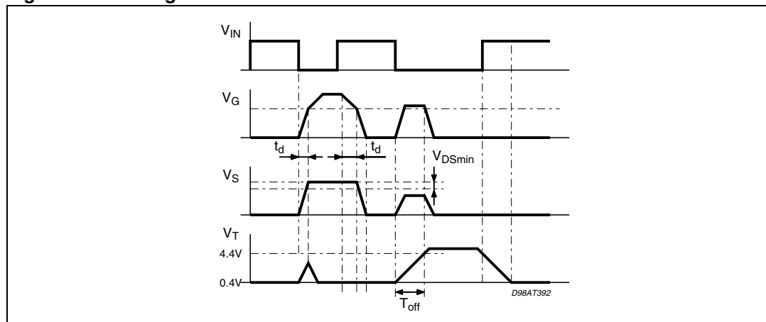
Figure 3. Timing characteristic
