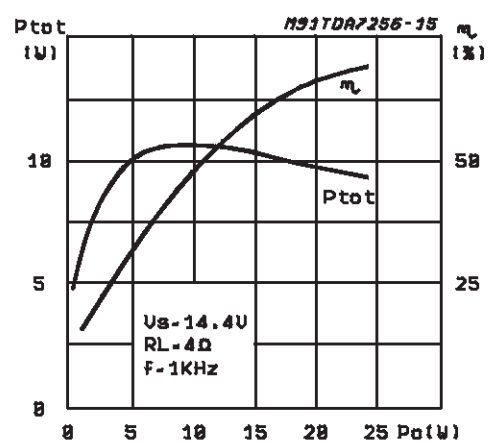
Figure 16: Power Dissipation &amp; Efficiency vs. Output Power
