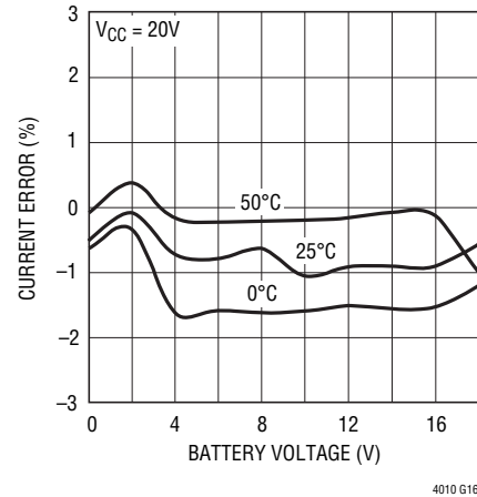
Fast Charge Current Output Regulation
