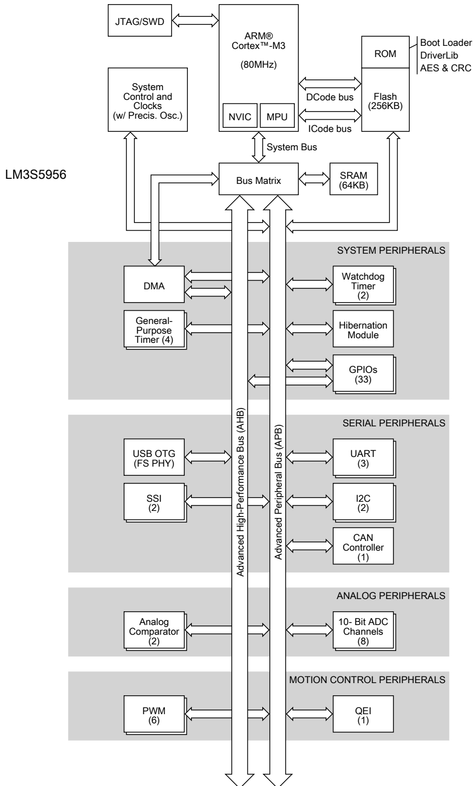
Figure 1-1. Stellaris LM3S5956 Microcontroller High-Level Block Diagram
