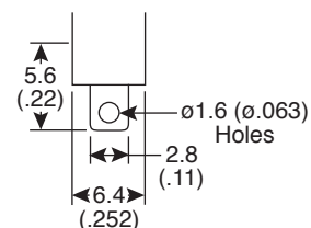
Solder Terminals
