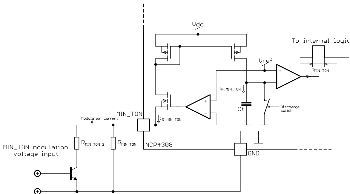
Figure 48. Possible Connection for MIN_T ON and MIN_T OFF Modulation
