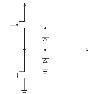
Figure 3-7: Indicator Outputs: SD/H \overline{D} , LOCKED, LOS
