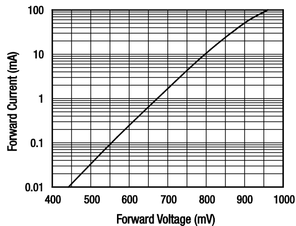
Figure 4. DC Characteristic
