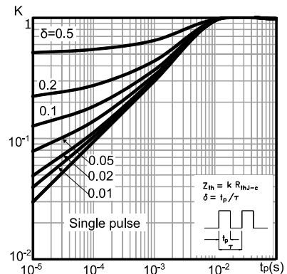
Figure 3: Thermal impedance
