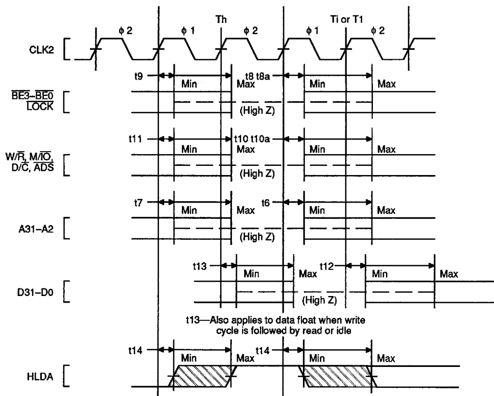
Figure 13. Output Float Delay and HLDA Valid Delay Timing
