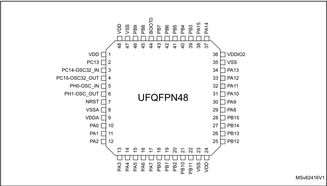
Figure 6. STM32L051x6/8 UFQFPN48
