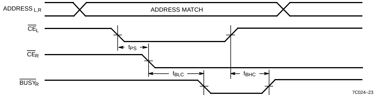
\overline{CE}_R Valid First:
