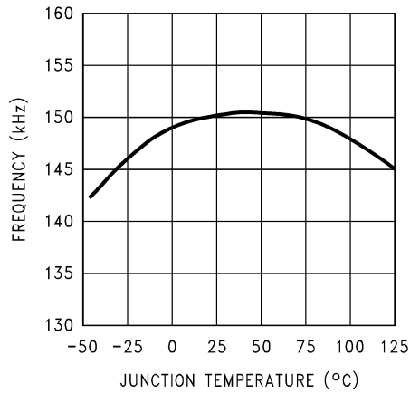
Figure 7-12. Switching Frequency
