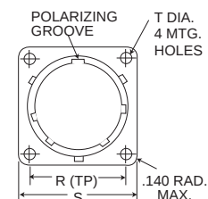
RECEPTACLE ASSEMBLY
