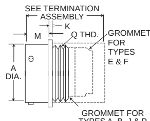
CRIMP KPSE00/MS3120
