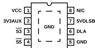
ISL6506BIBZ (8 LD EPD SOIC) TOP VIEW
