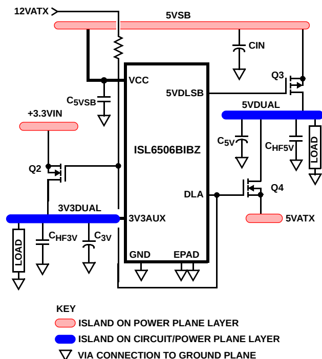
FIGURE 4. PRINTED CIRCUIT BOARD ISLANDS
