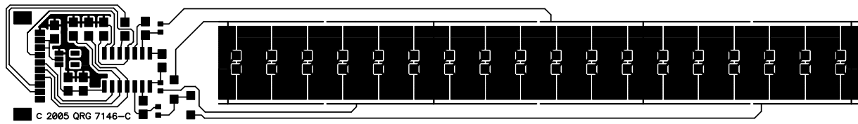
Figure 1-3 Conventional PCB Layout (1-sided) Copper side faces away from the panel; the bare side is glued to the inside of the product.
