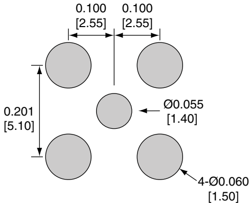
RECOMMENDED FOOTPRINT
