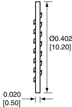
WASHER
