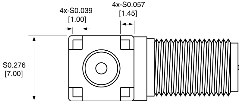
BOTTOM VIEW
