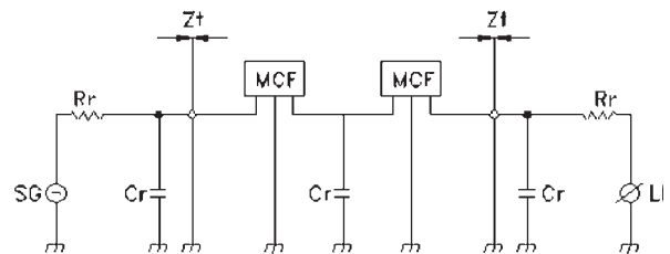
Figure 2 4 Pole MCF
