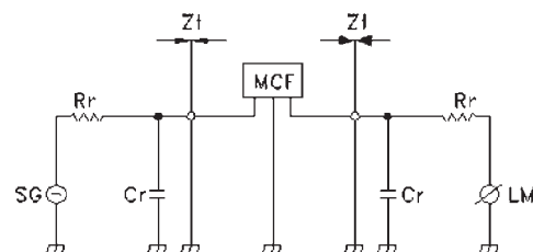
Figure 3 4 Pole MCF
