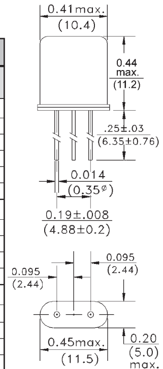
HC49U3 Package Configuration
