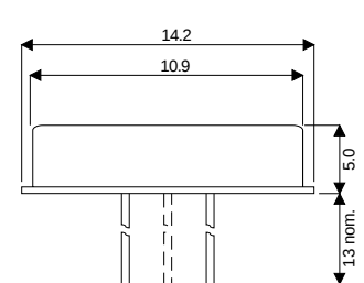
Lensed TO-39
