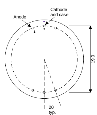
TO-M
