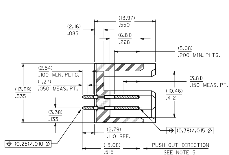
SECTION W-W
