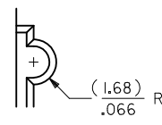
DETAIL "S"
