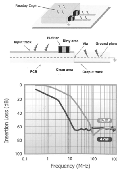
Figure 2. Improved shielding
